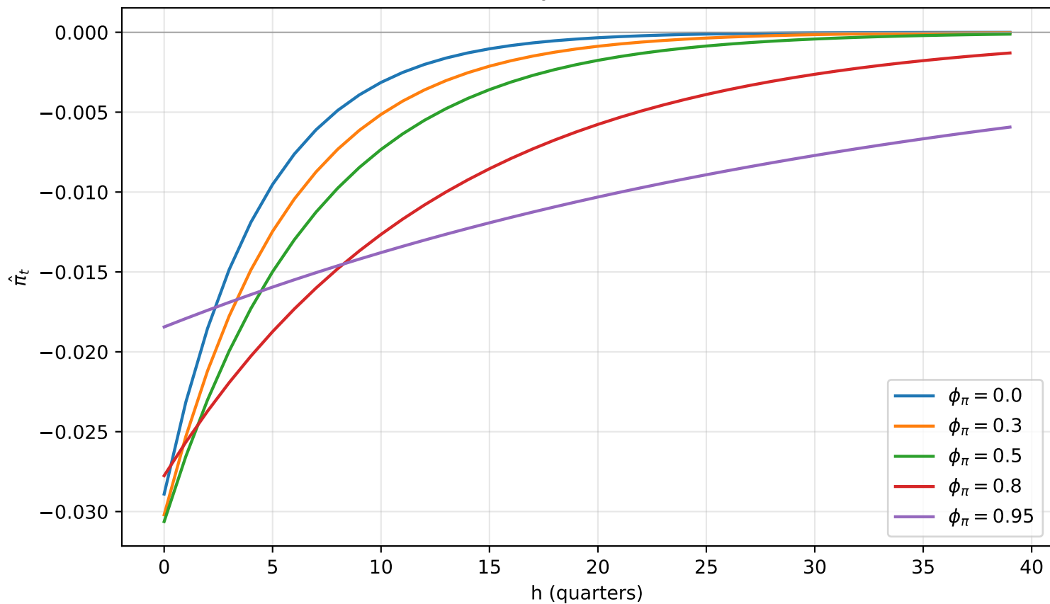
Sensitivity of \hat{\pi} to \hat{\lambda}^L shock
