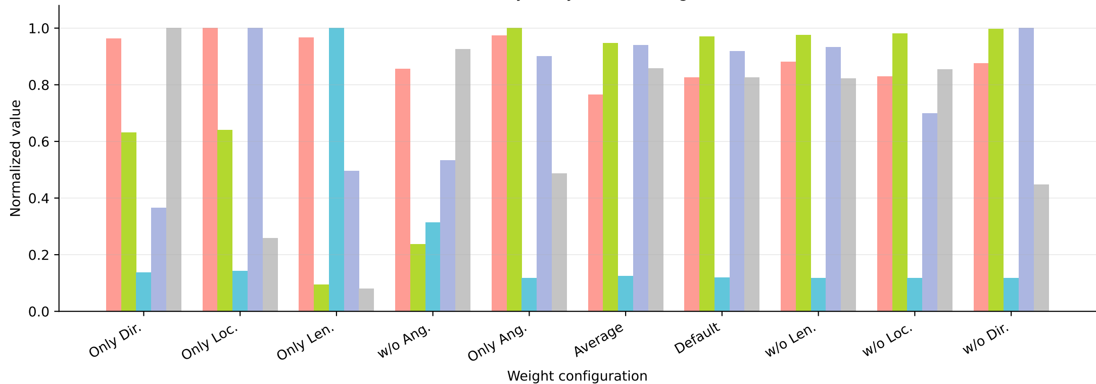
Sensitivity Analysis of VP Weights
