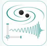
Gravitational-wave detection
