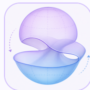
Sphere eversion
