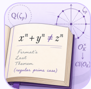
Fermat (regular case)
