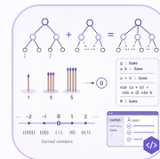
Combinatorial games
