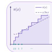
Prime Number Theorem
