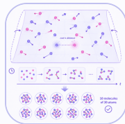
Molecular self-assembly
