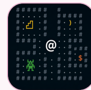
NetHack
