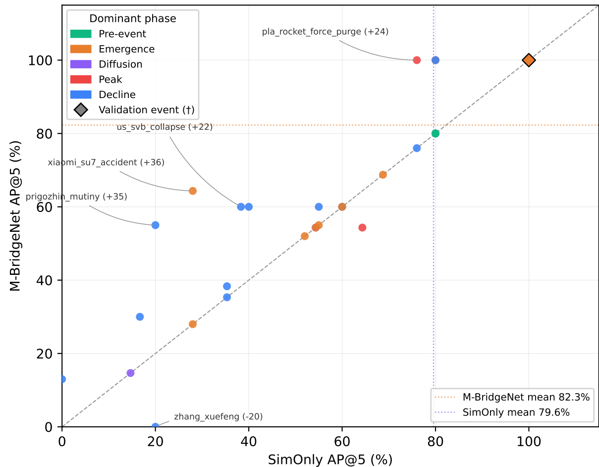
Per-event AP@5: M-BridgeNet vs SimOnly (67-event CPHot test set; colored by dominant lifecycle phase)
