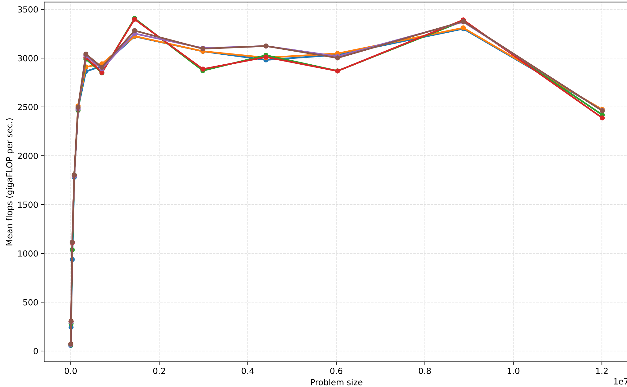
Apps_VOL3D throughput - Mean flops (gigaFLOP per sec.)
