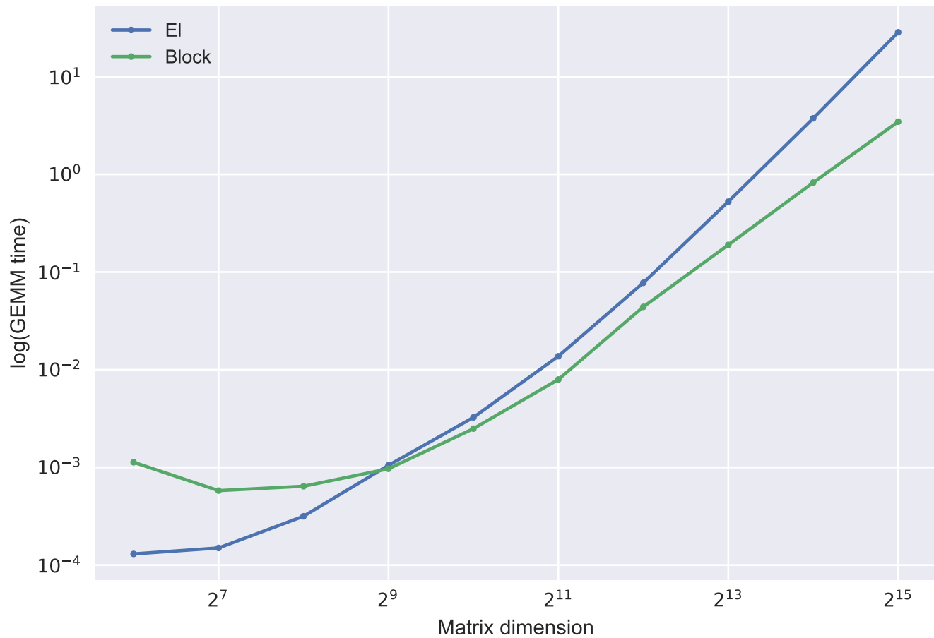
El vs Block GEMM time, default blocksize, 48 procs, 4 nodes, Catalyst
