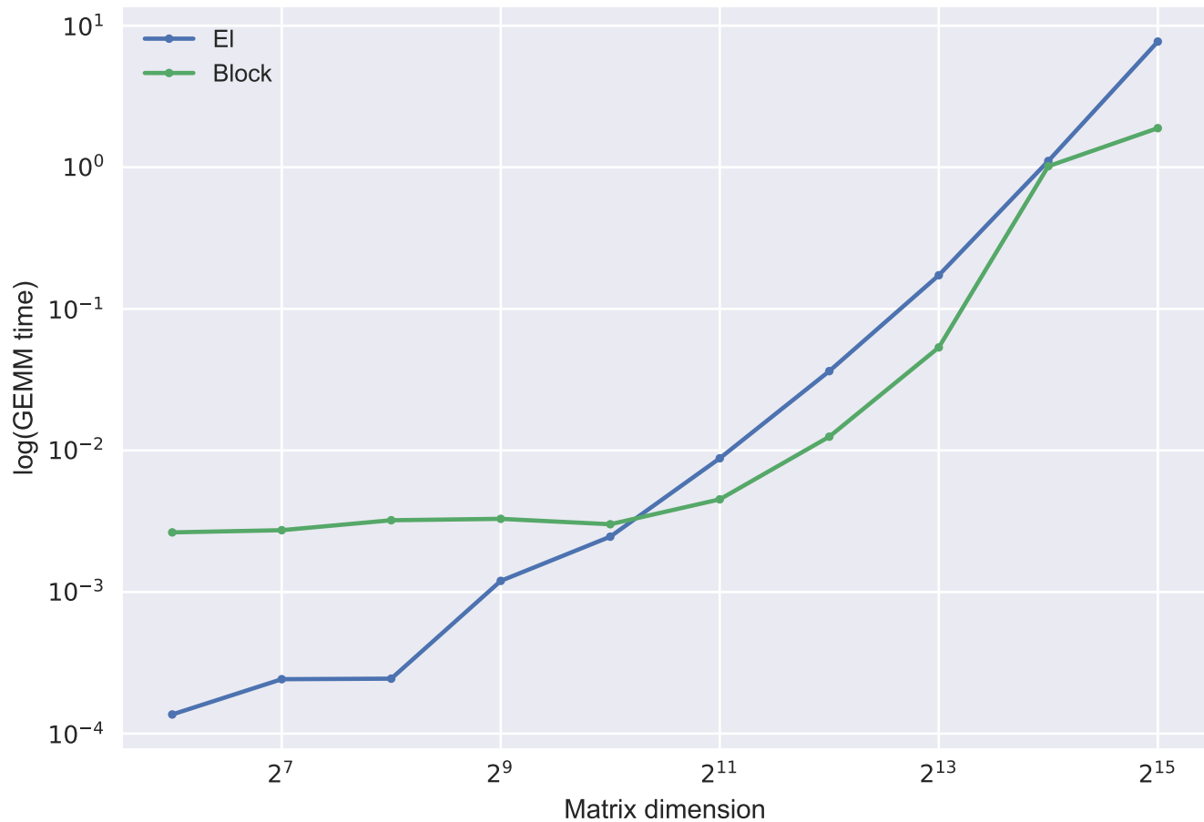
EI vs Block GEMM time, default blocksize, 192 procs, 16 nodes, Catalyst
