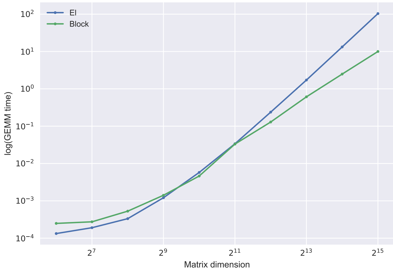
El vs Block GEMM time, default blocksize, 12 procs, 1 nodes, Catalyst
