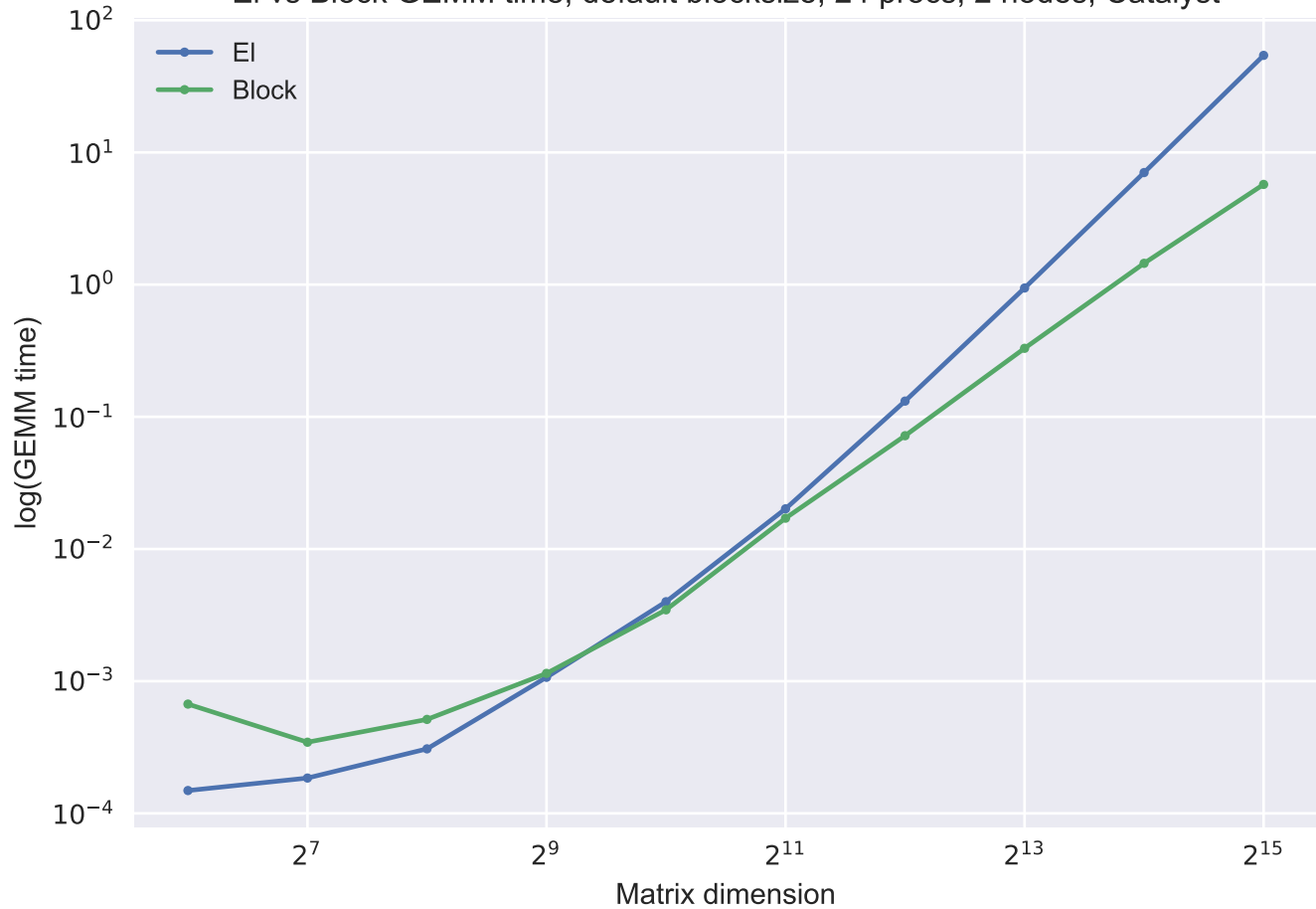
El vs Block GEMM time, default blocksize, 24 procs, 2 nodes, Catalyst
