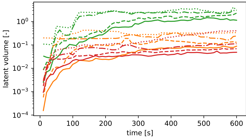
latent dynamics
