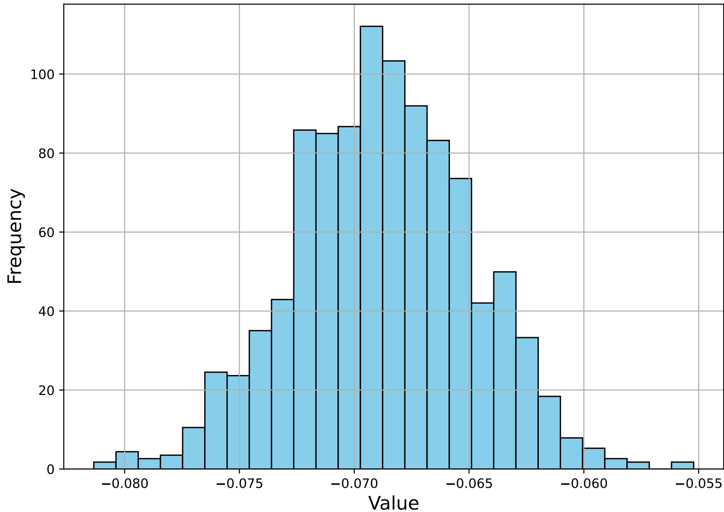
Variable 0, feature 10: x_1 x_0^{(0.875)}
