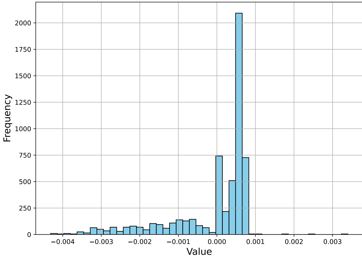
Variable 0, feature 11: \max(0, x_0 - a)
