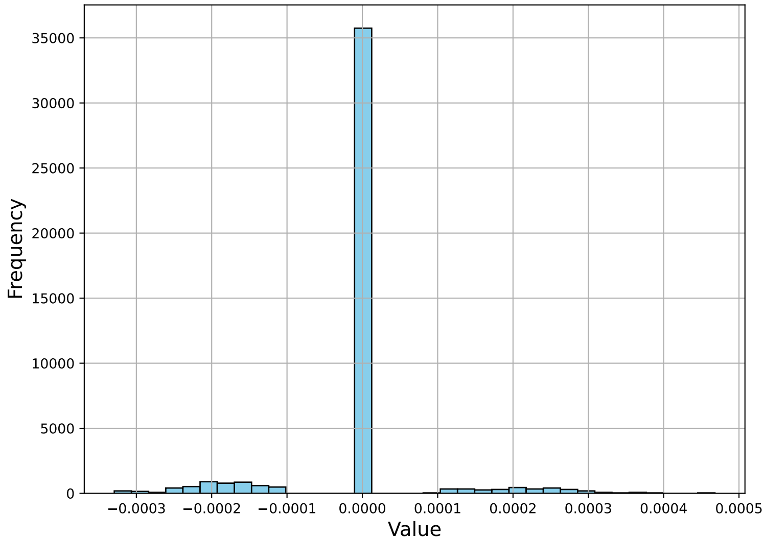
Variable 1, feature 2: x_0^2
