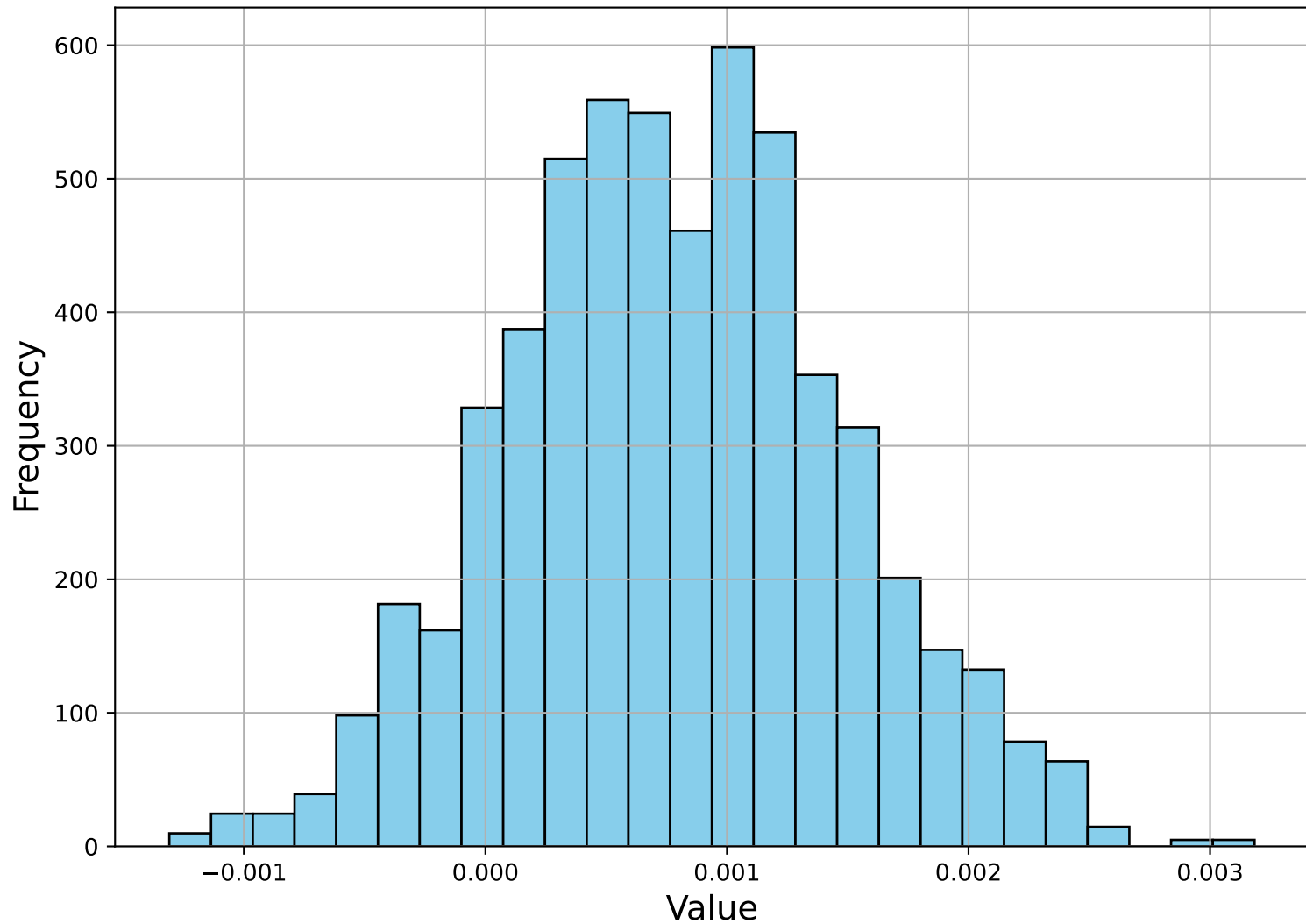
Variable 1, feature 12: \max(0, x_1 - a)
