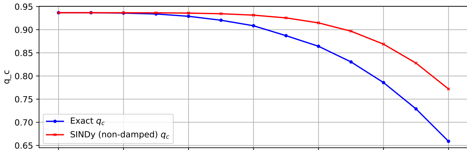
Trajectory 1007 (non-damped)
