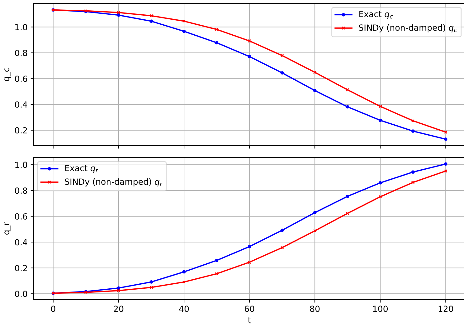
Trajectory 1013 (non-damped)
