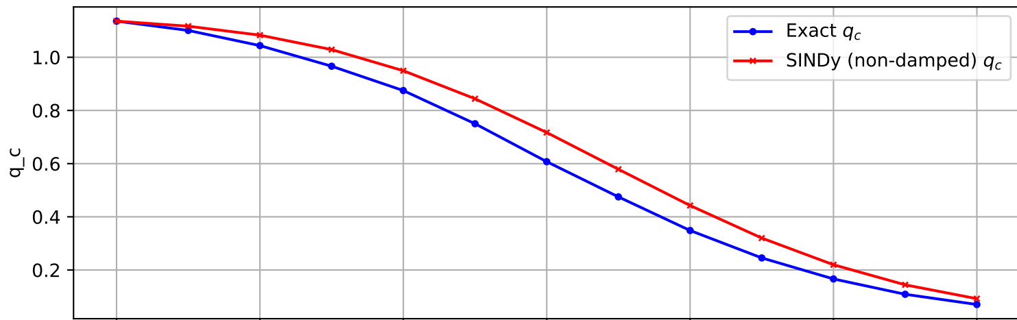
Trajectory 1017 (non-damped)
