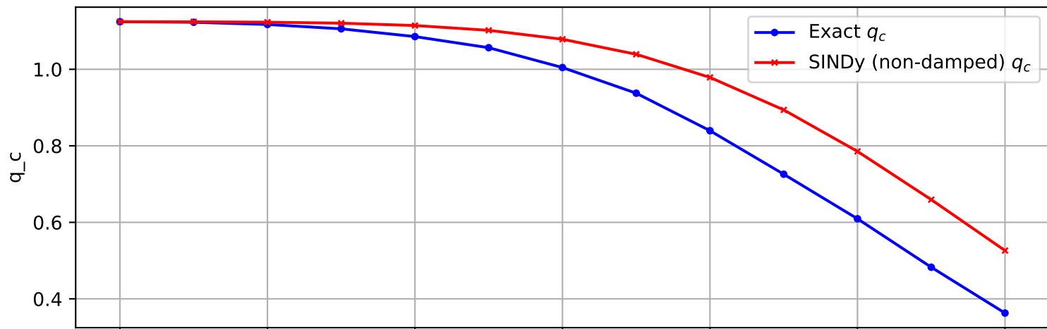
Trajectory 1032 (non-damped)
