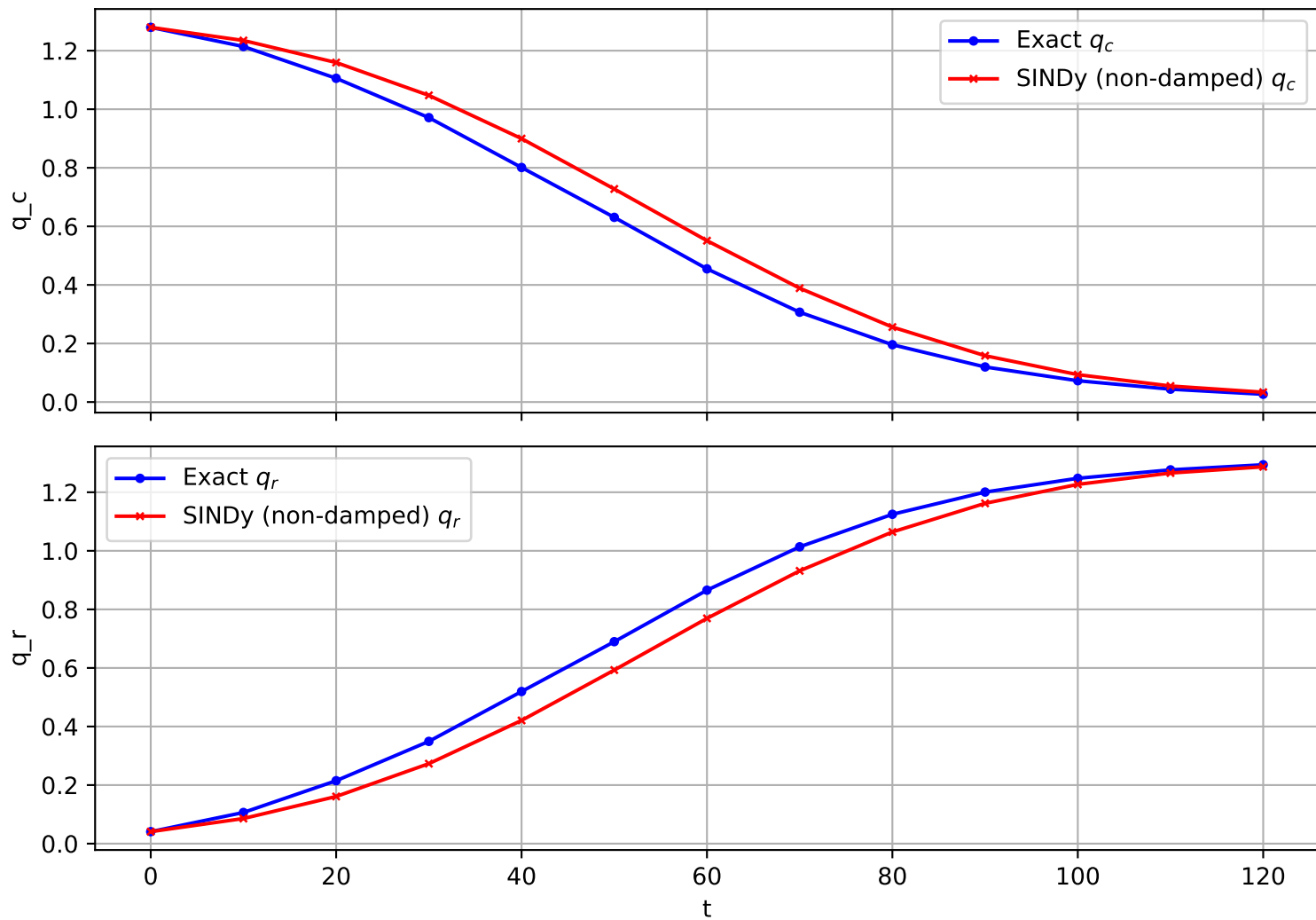
Trajectory 1053 (non-damped)
