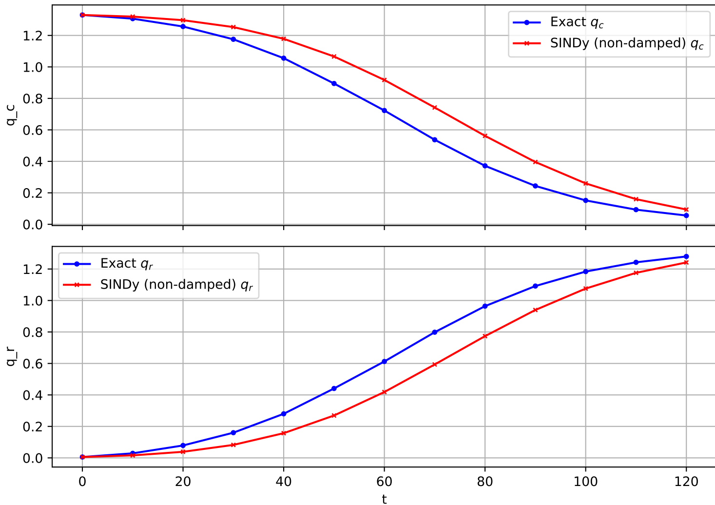
Trajectory 1059 (non-damped)
