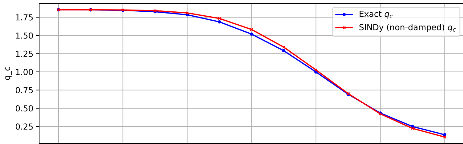
Trajectory 106 (non-damped)
