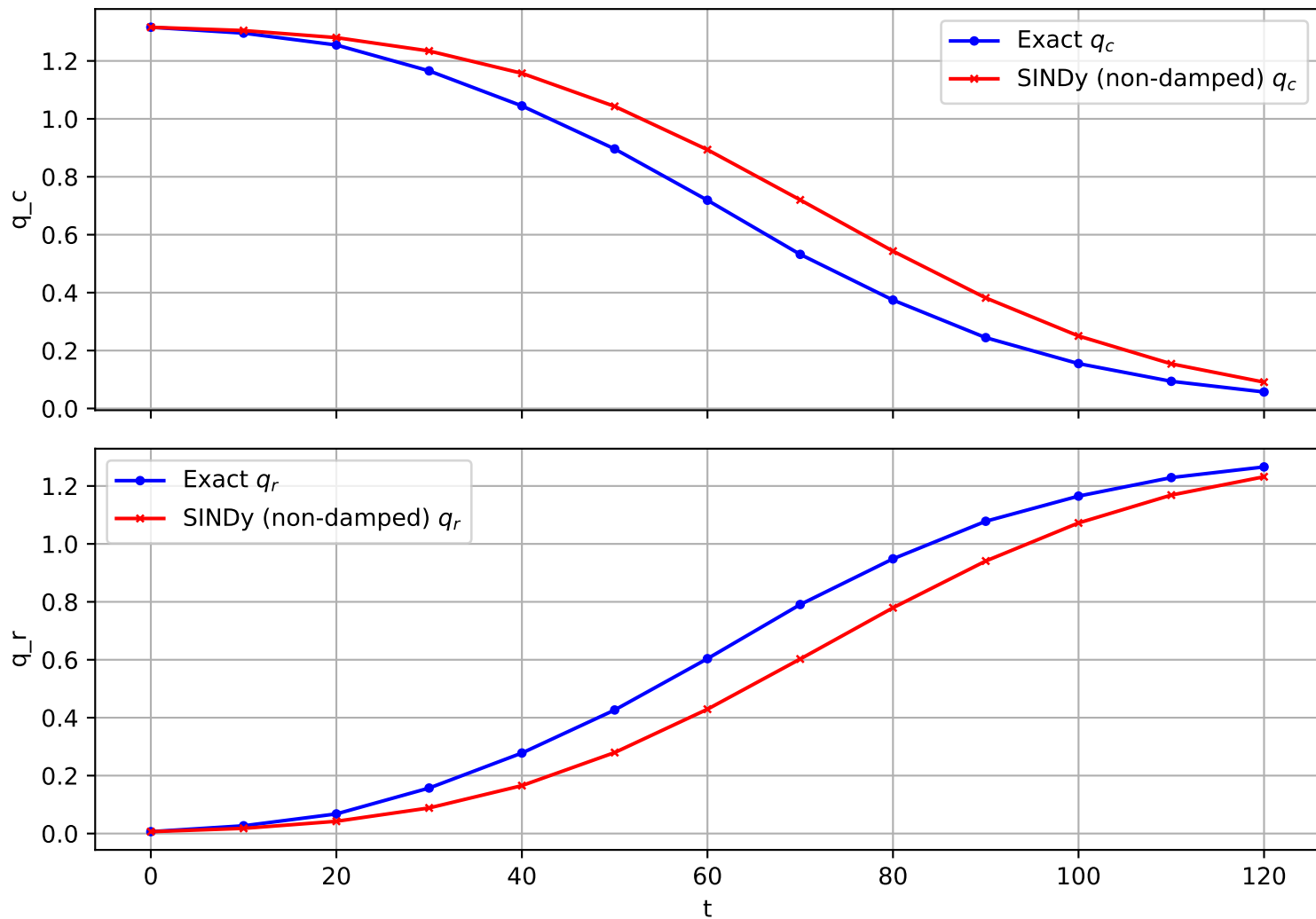
Trajectory 1060 (non-damped)
