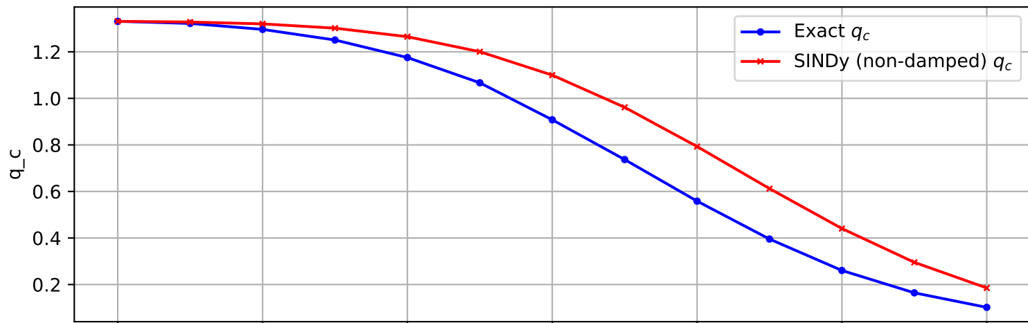
Trajectory 1064 (non-damped)
