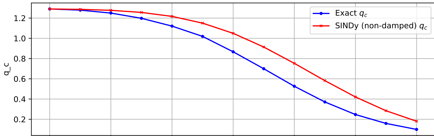
Trajectory 1072 (non-damped)
