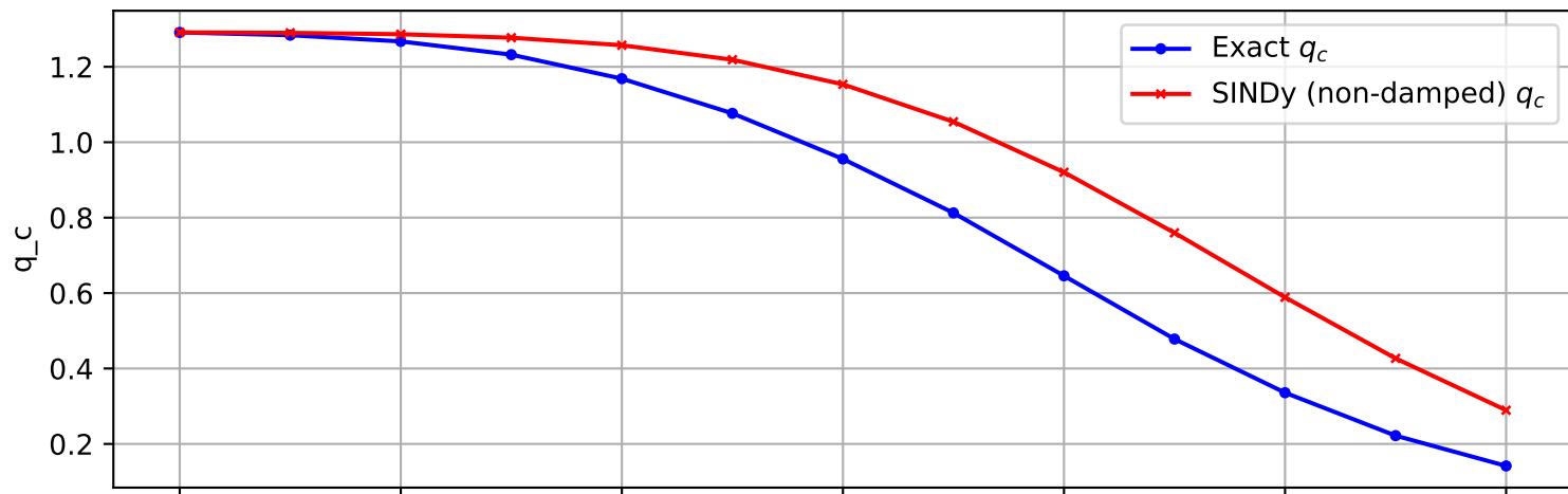
Trajectory 1078 (non-damped)
