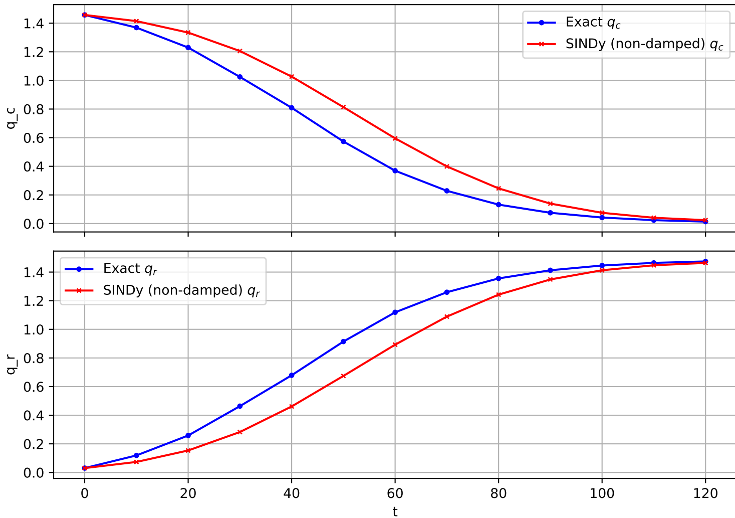
Trajectory 1083 (non-damped)
