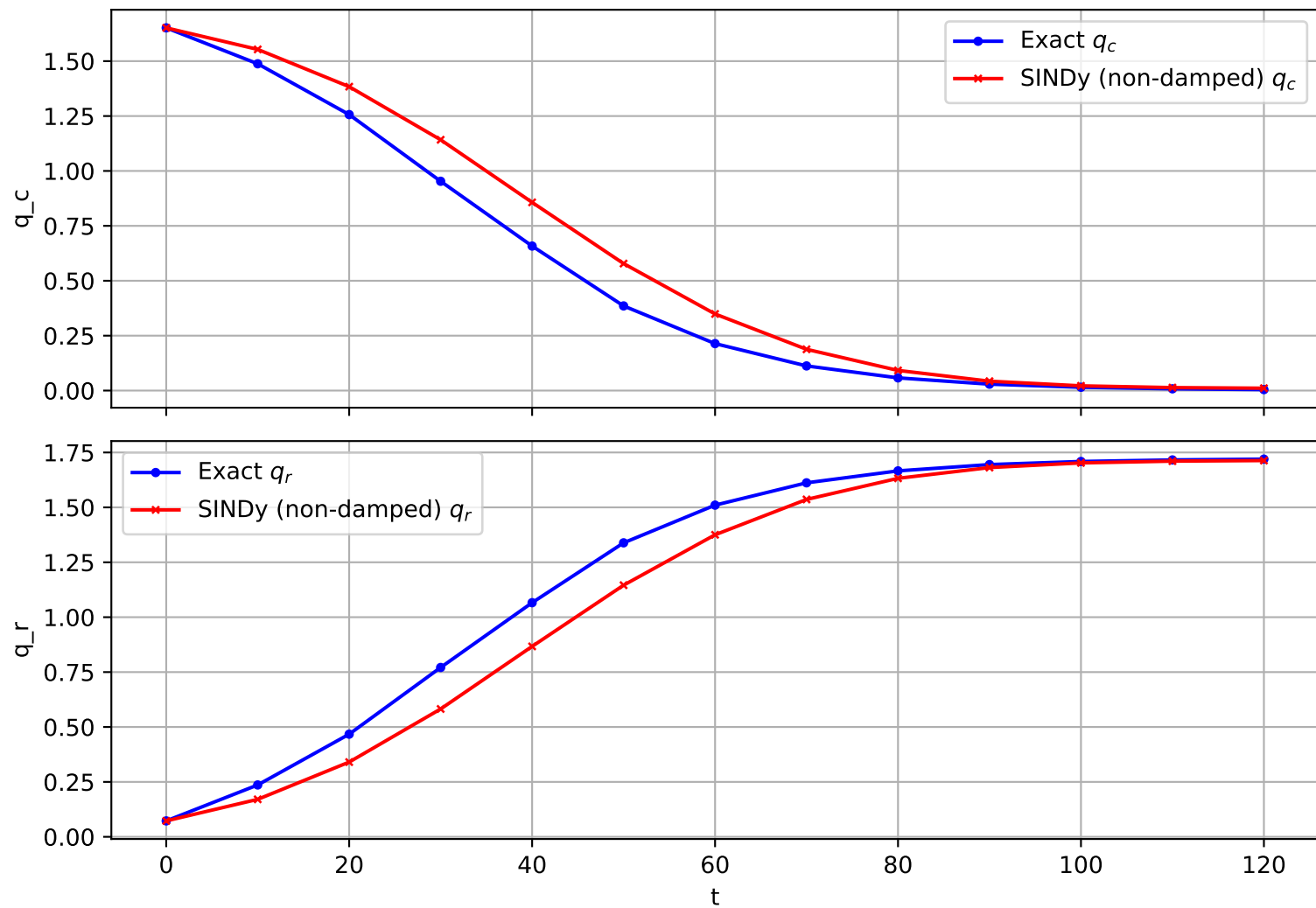
Trajectory 1114 (non-damped)
