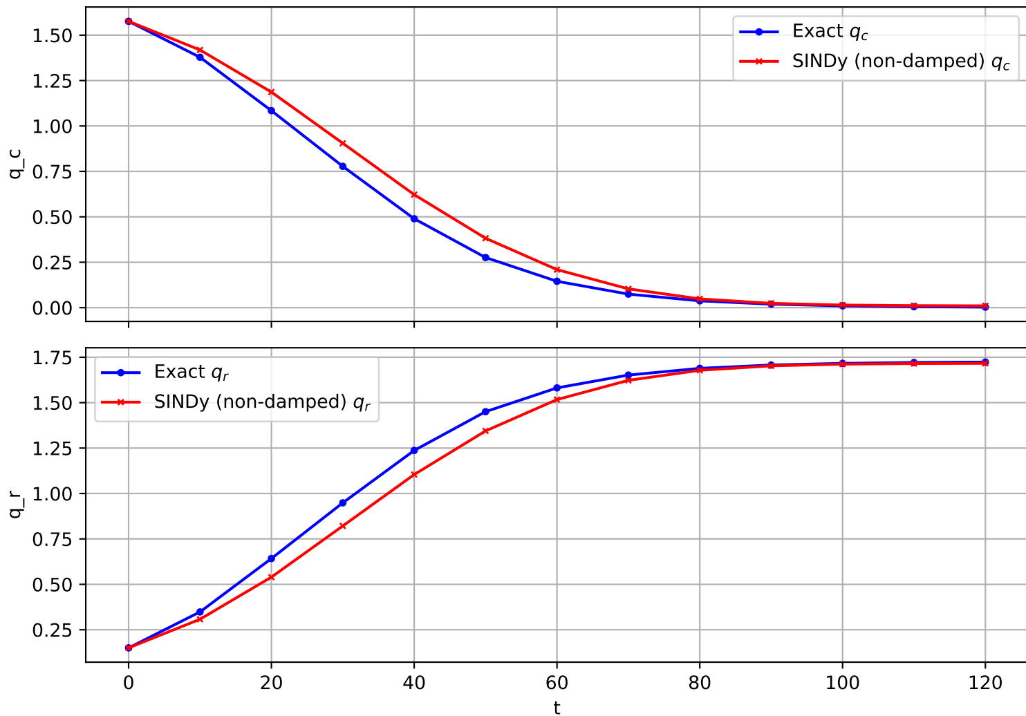
Trajectory 1119 (non-damped)
