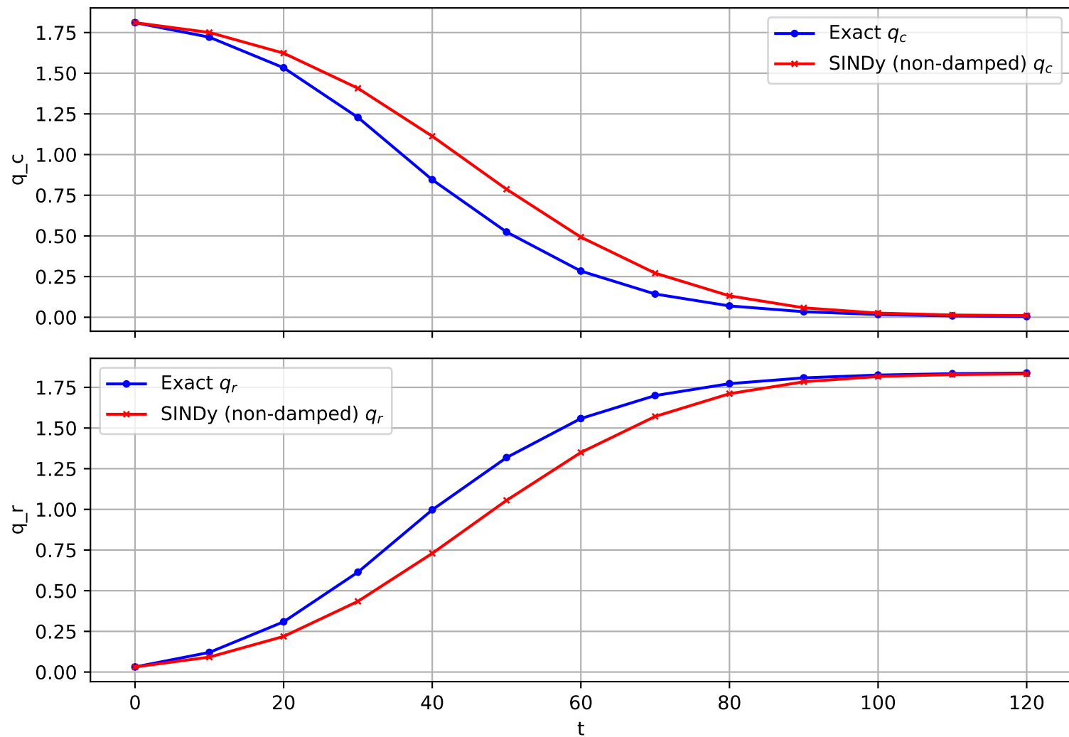
Trajectory 1125 (non-damped)
