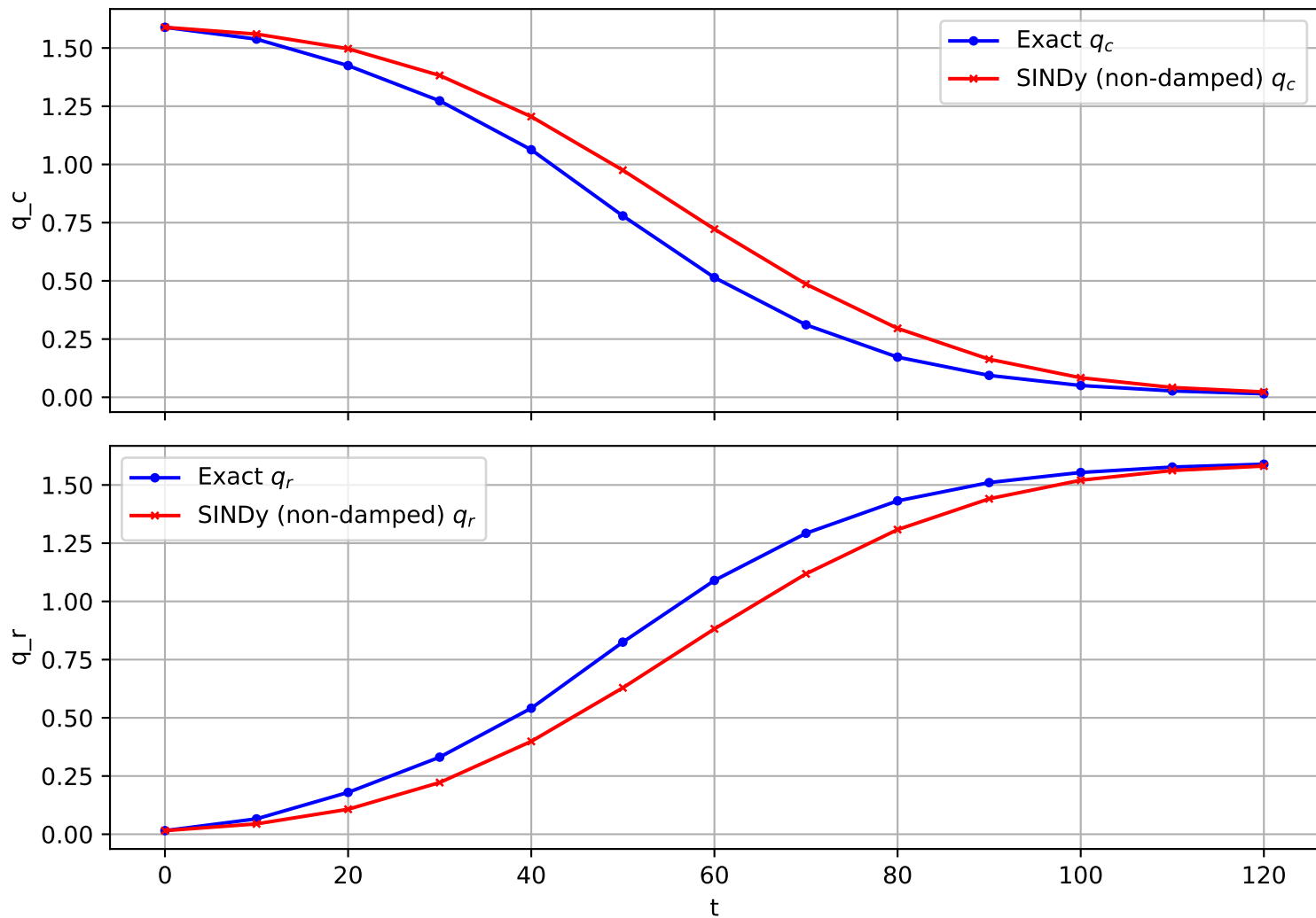
Trajectory 1140 (non-damped)
