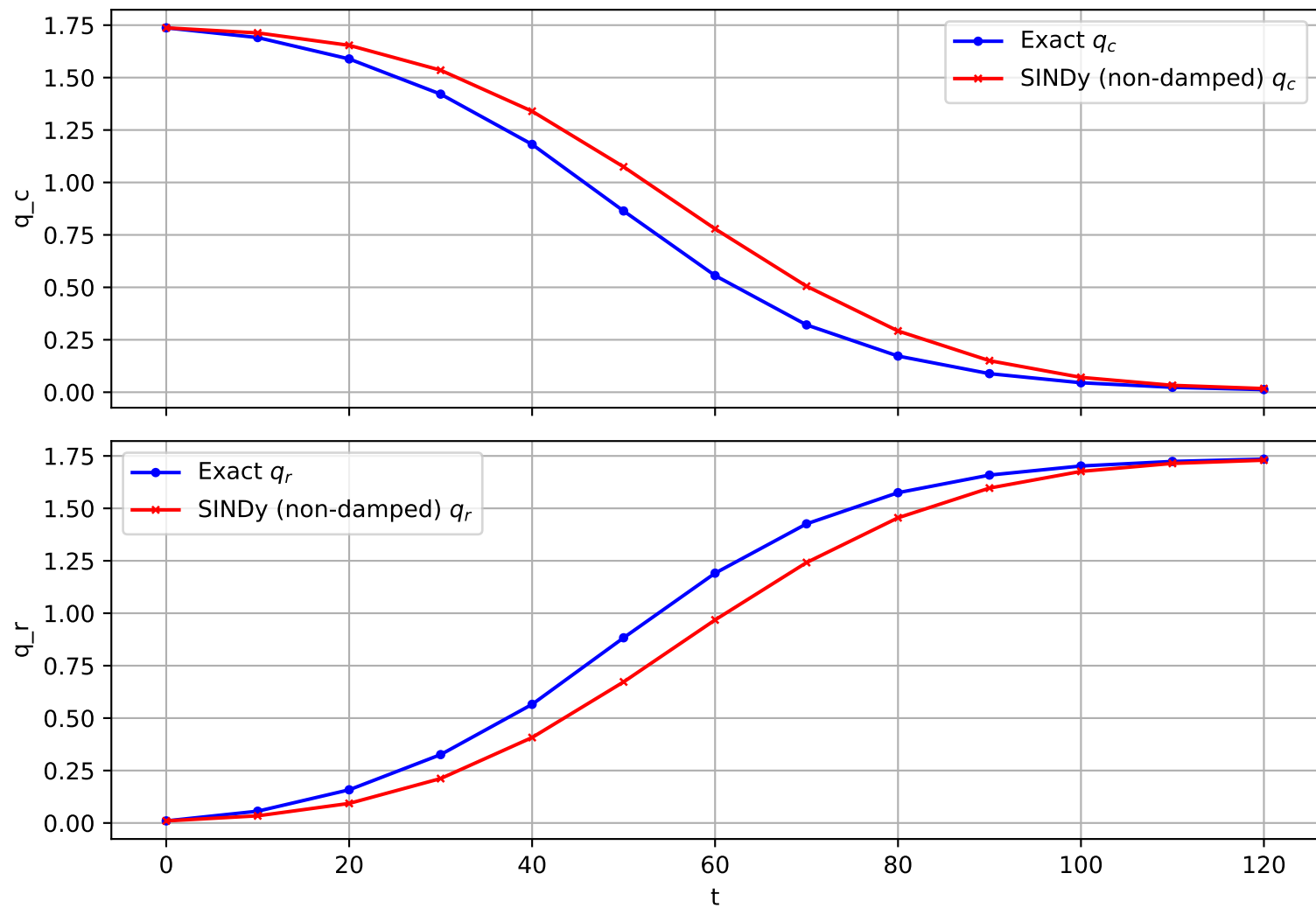
Trajectory 1147 (non-damped)
