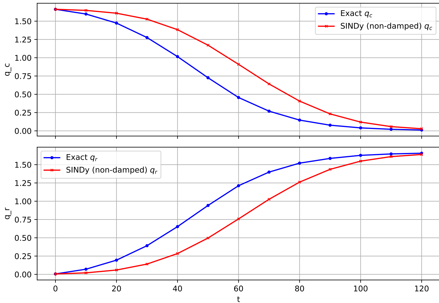
Trajectory 1148 (non-damped)
