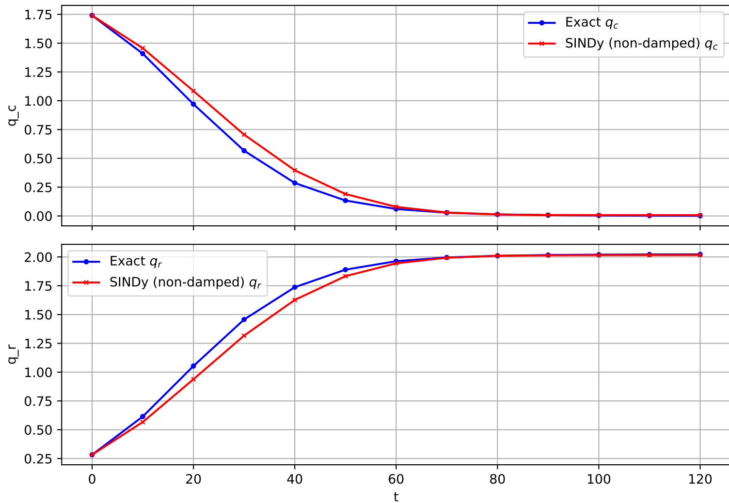
Trajectory 1155 (non-damped)
