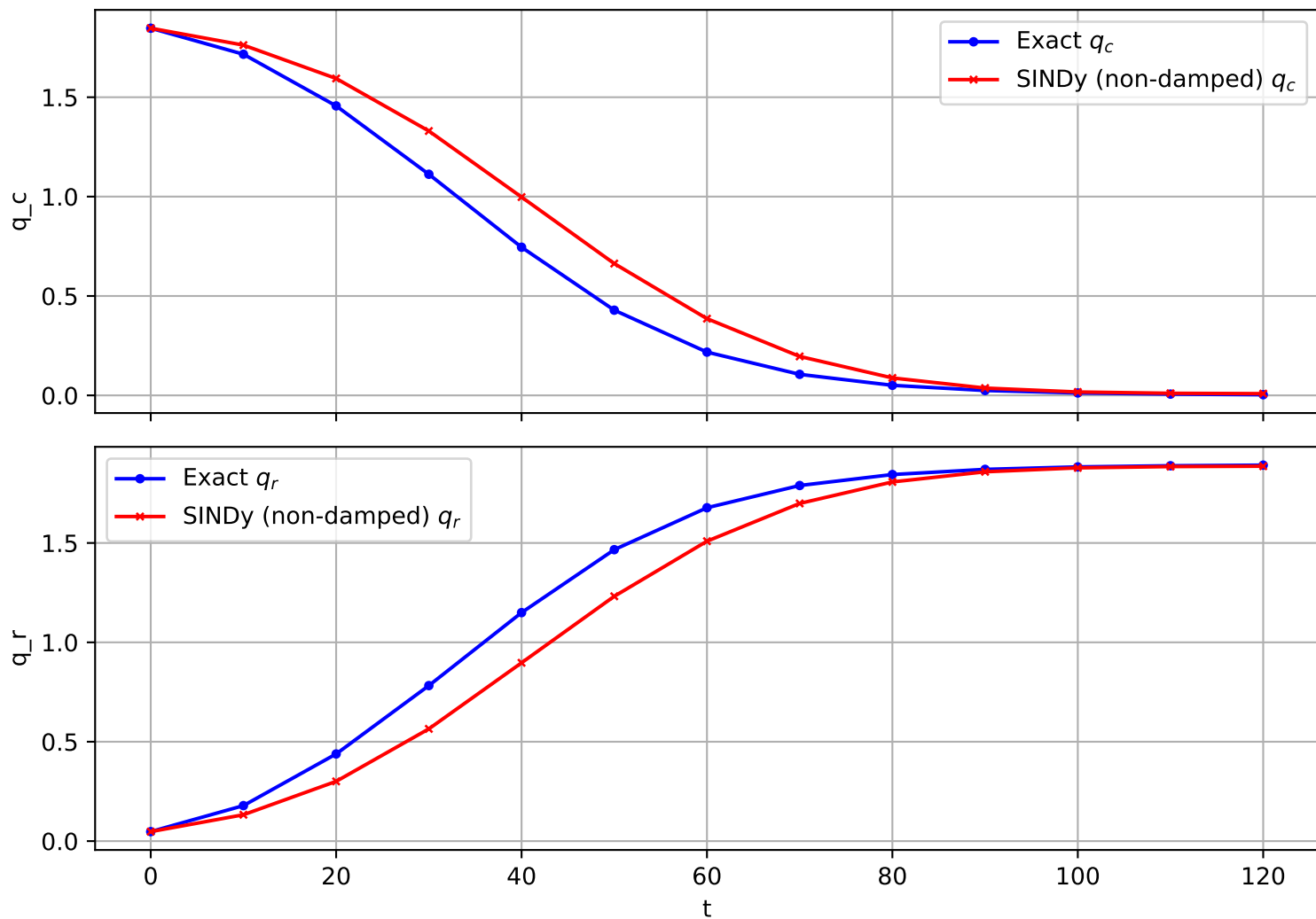
Trajectory 1162 (non-damped)
