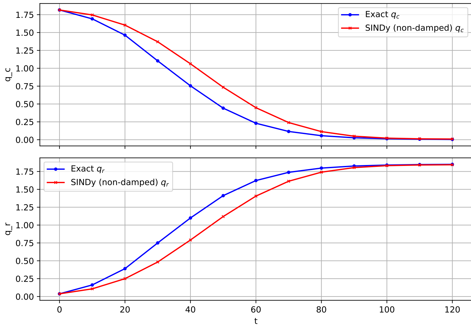
Trajectory 1174 (non-damped)
