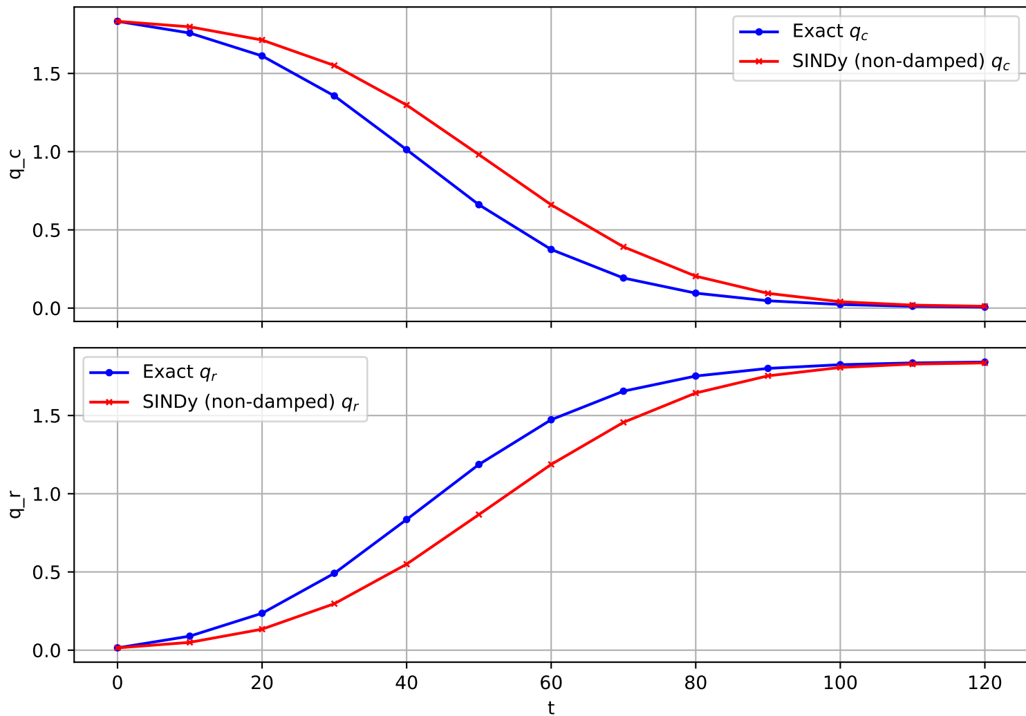
Trajectory 1182 (non-damped)
