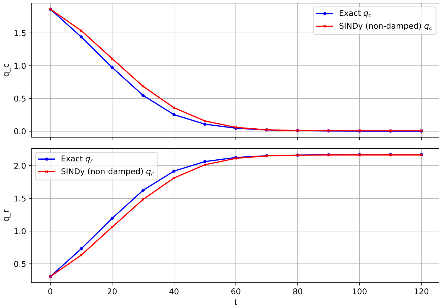
Trajectory 1185 (non-damped)
