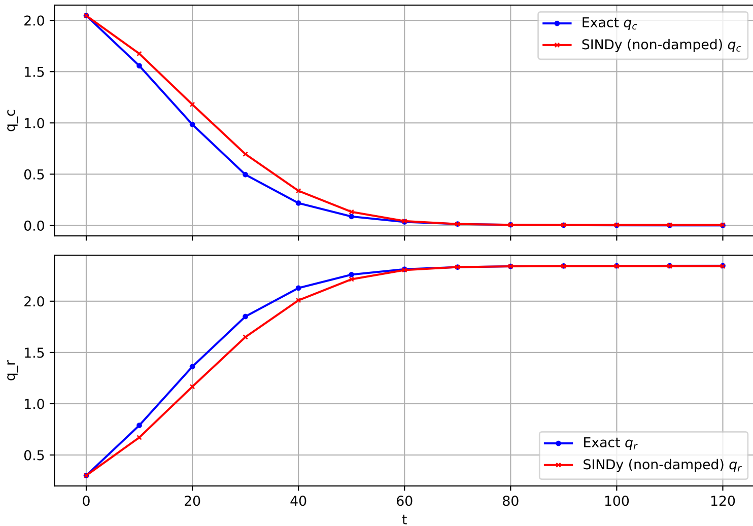
Trajectory 1187 (non-damped)
