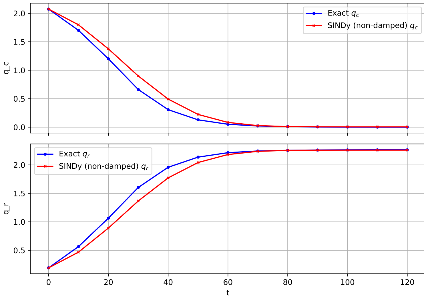
Trajectory 1202 (non-damped)
