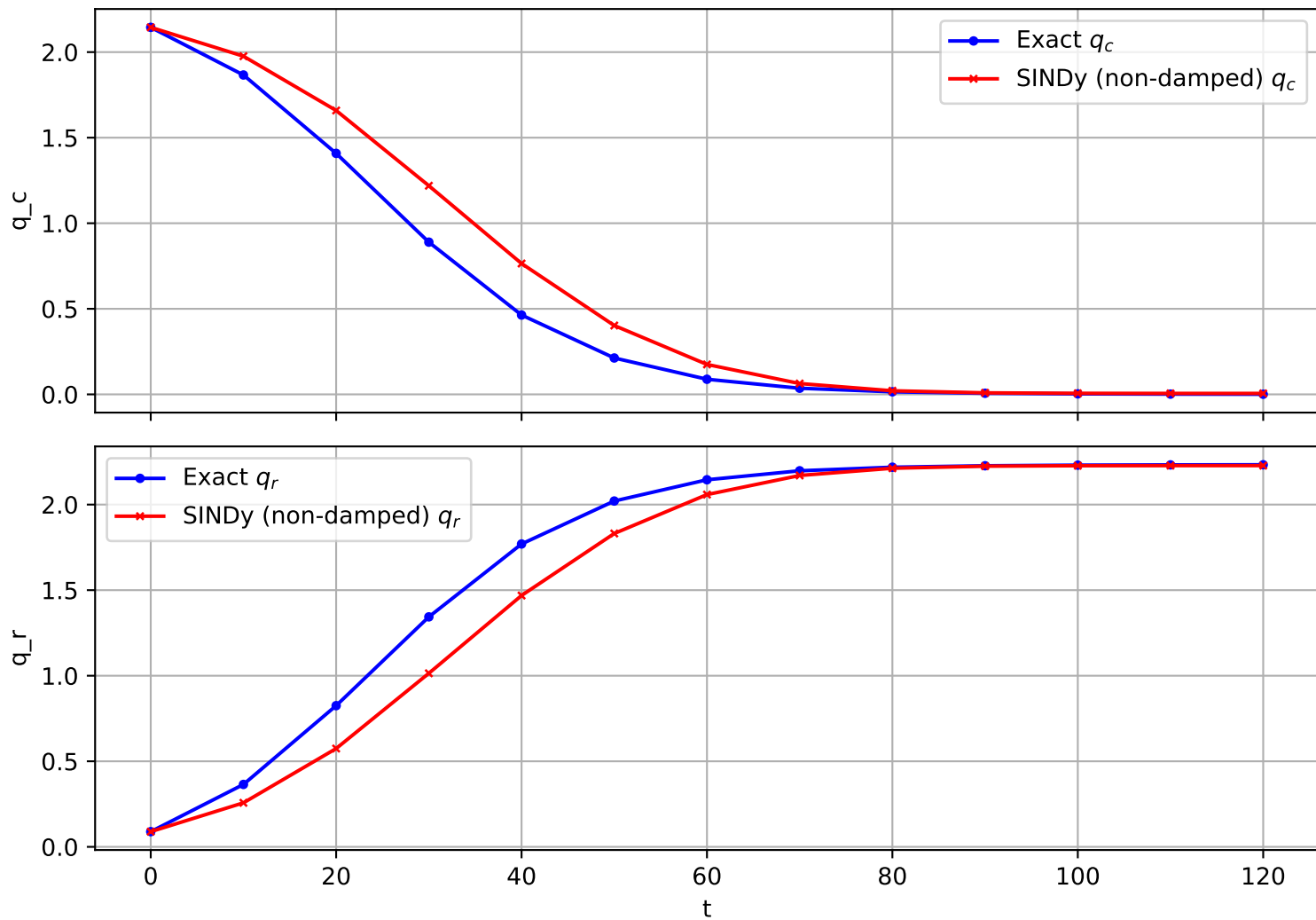
Trajectory 1208 (non-damped)
