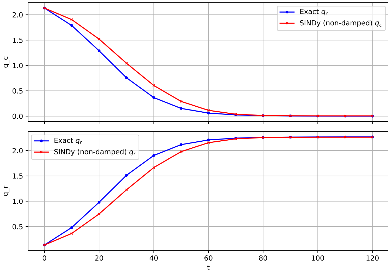
Trajectory 1210 (non-damped)
