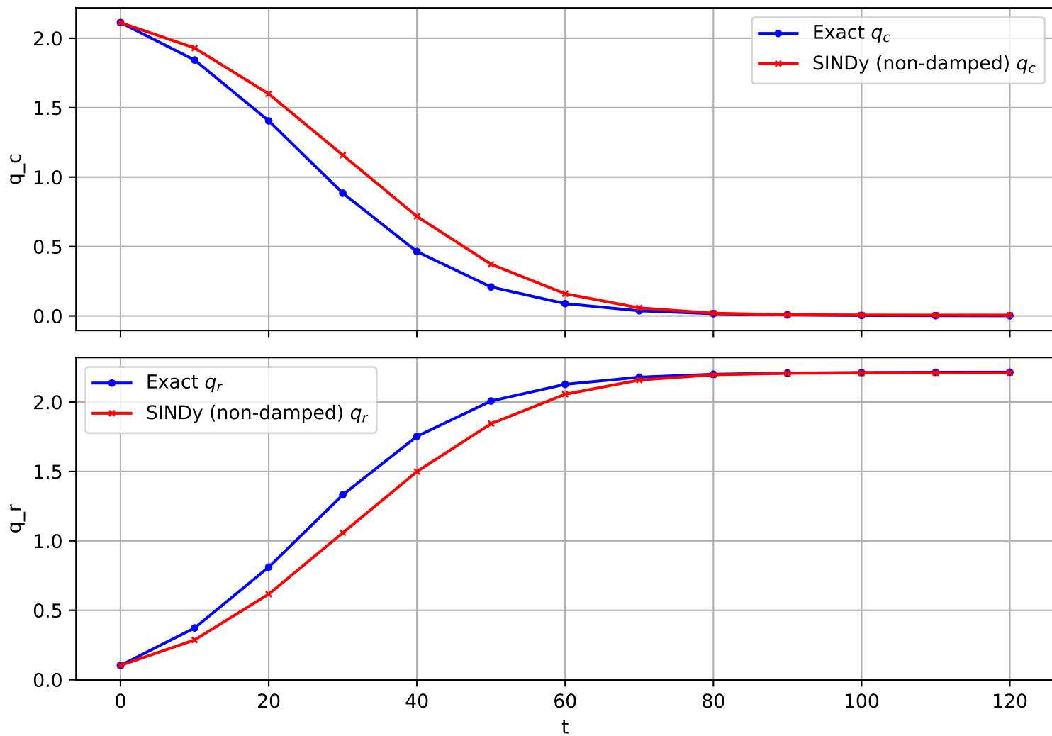
Trajectory 1211 (non-damped)
