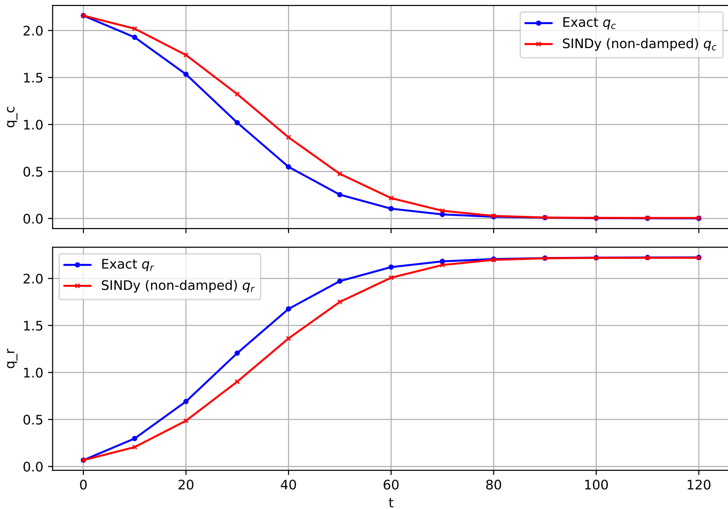
Trajectory 1214 (non-damped)
