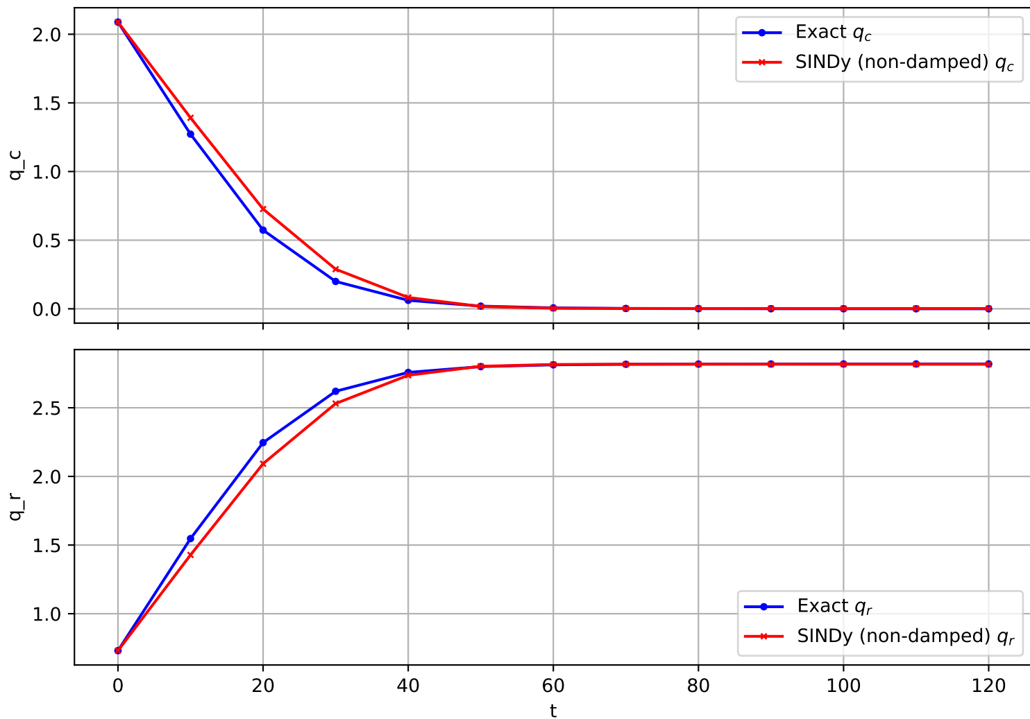
Trajectory 1221 (non-damped)
