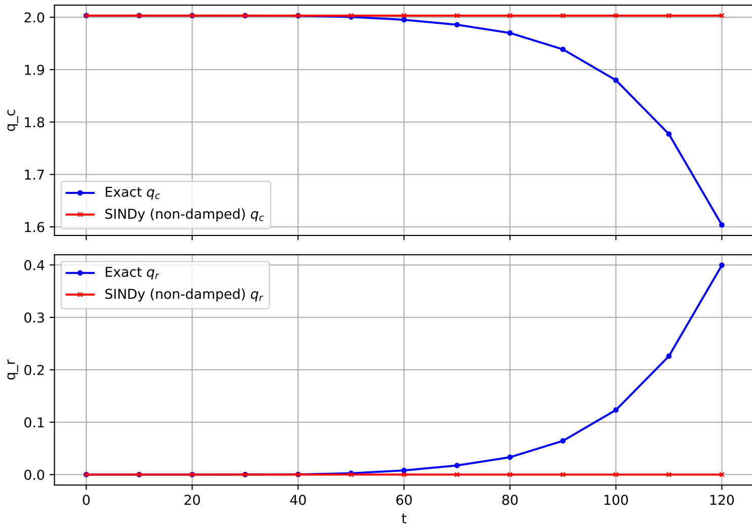
Trajectory 123 (non-damped)
