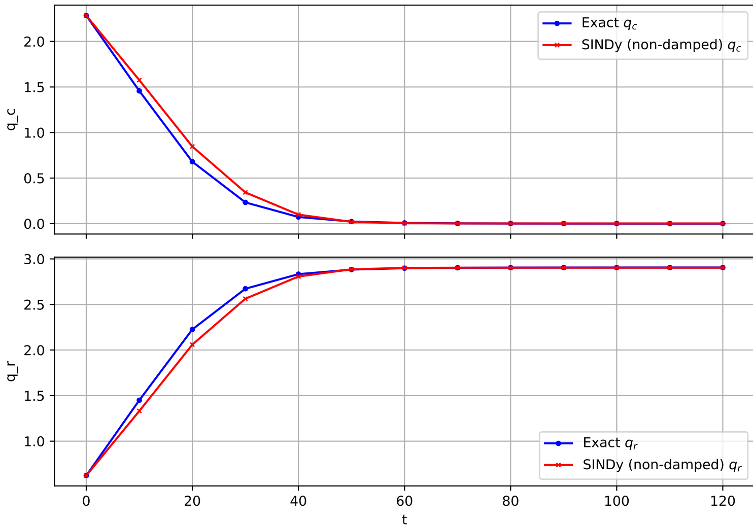
Trajectory 1234 (non-damped)
