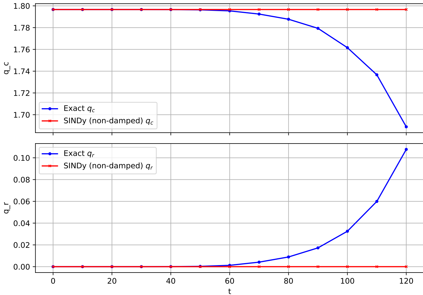
Trajectory 125 (non-damped)
