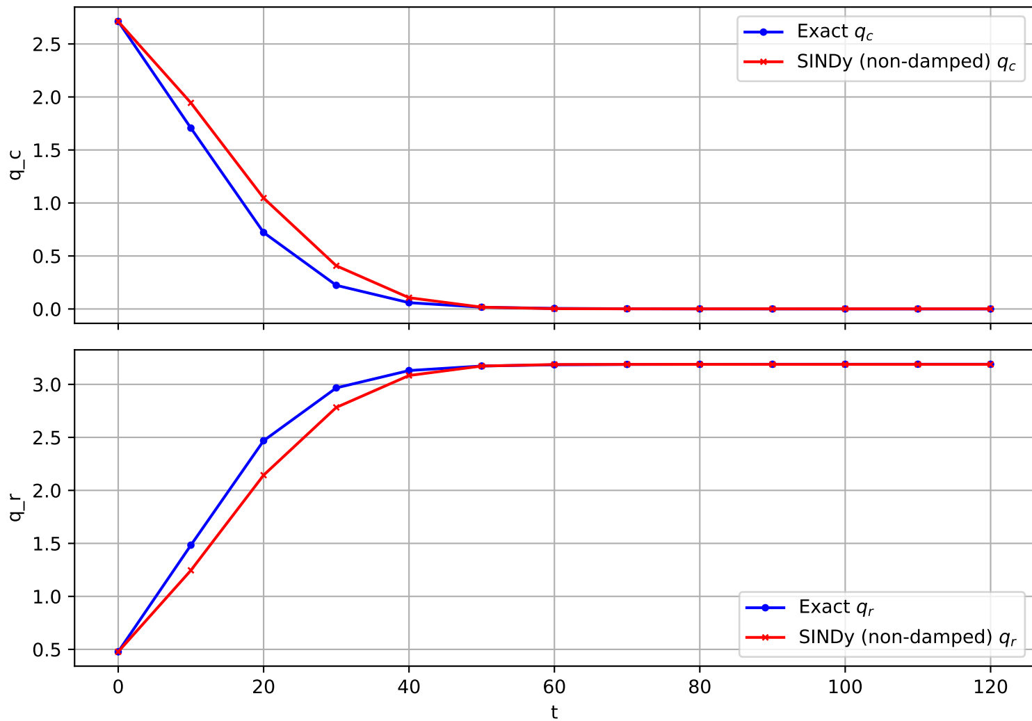
Trajectory 1274 (non-damped)
