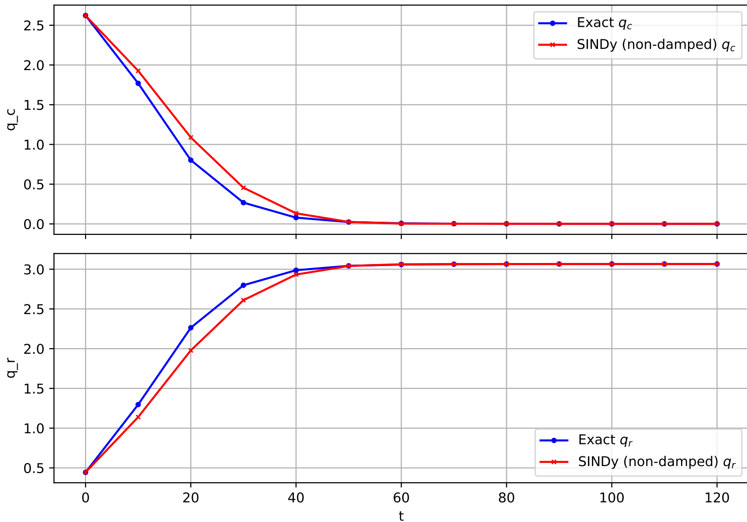
Trajectory 1277 (non-damped)
