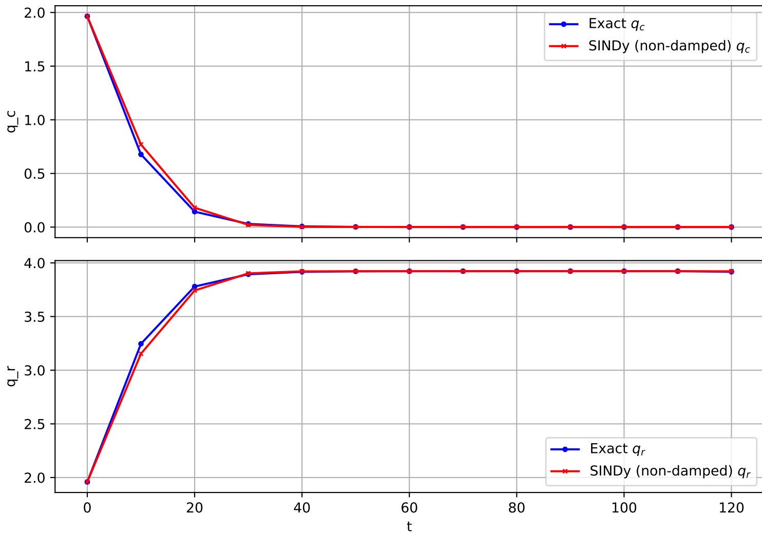
Trajectory 1290 (non-damped)
